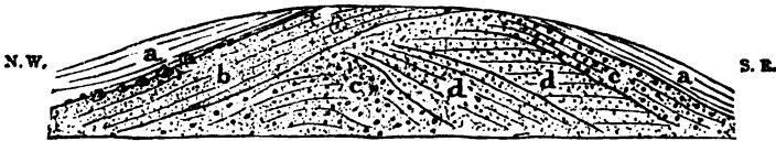
FIG. 88.—Section of kame near Dover, New Hampshire. Length, three hundred feet; height forty feet; base, about forty feet above the Cochecho River, or seventy-five feet above the sea. a, a , gray clay; b , fine sand; c, c , coarse gravel containing pebbles from six inches to one foot and a half in diameter; d, d , fine gravel. (Upham.)
